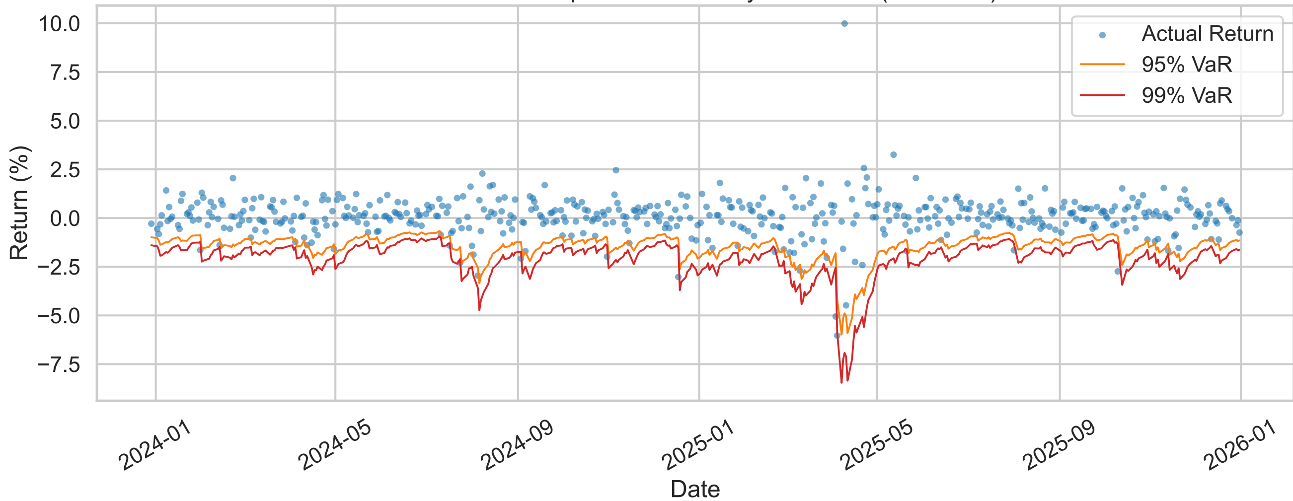
SPY Out-of-Sample Returns vs Dynamic VaR (EGARCH)
